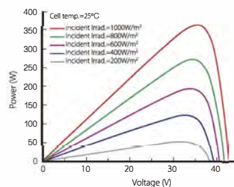
Power-Voltage Curve (LR4-60HPB-360M)
